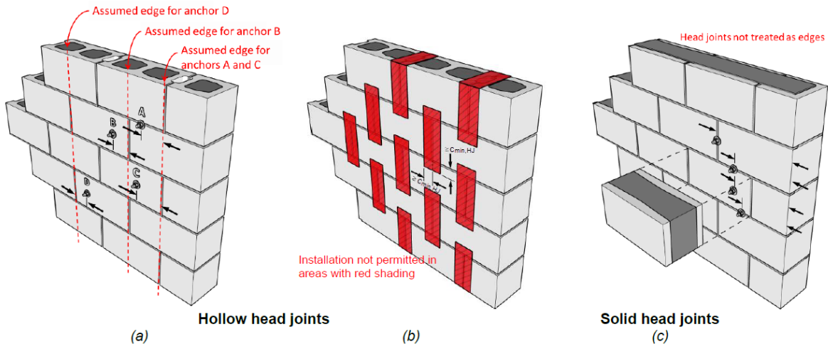
FIGURE 7—(a) Edge distance considerations in fully grouted CMU construction with hollow head joints, (b) exclusion zones in fully grouted construction with hollow head joints, and (c) edge distance considerations in fully grouted CMU construction with solid head joints. Note: dimensions to upper and lower edges omitted for clarity.
